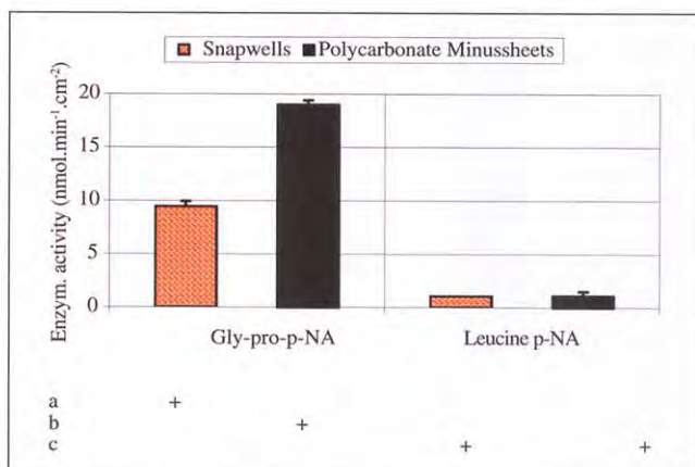
Fig. 4: Dipeptidase (DP) and aminopeptidase (AP) activities of Caco-2 cells seeded on Snapwells or polycarbonate Minucells (Minusheets). Caco-2 cells (passage 63) were seeded on Snapwells or polycarbonate support filters mounted in Minusheets. The inserts were coated with 2.5 \mu\text{g}/\text{cm}^2 of collagen IV. The cells were allowed to grow according to the procedure described in the Experimental section and the enzymatic activities were determined. The bars represent the mean and standard deviation of 3 individual experiments. At the bottom of the graph, homogenous groups are identified using the letters a, b, and c. There are no statistically significant differences between data belonging to a homogenous group
