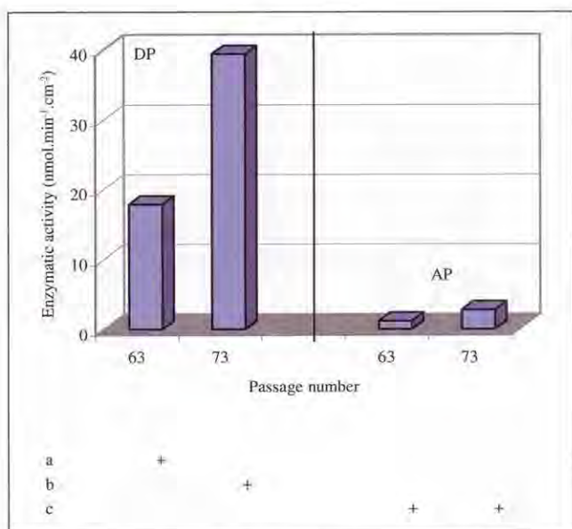
Fig. 7: The effect of passage number on dipeptidase (DP) and aminopeptidase (AP) activities of Caco-2 cells grown in the perfusion system. Caco-2 cells (passage numbers 63 and 73) were grown for 28 days in the perfusion system. The results represent the means of a pool of 9 polycarbonate support filters coated with 2.5, 5 and 10 \mu\text{g}/\text{cm}^2 of collagen IV.
